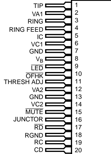
Figure 2 - Pin Connections
